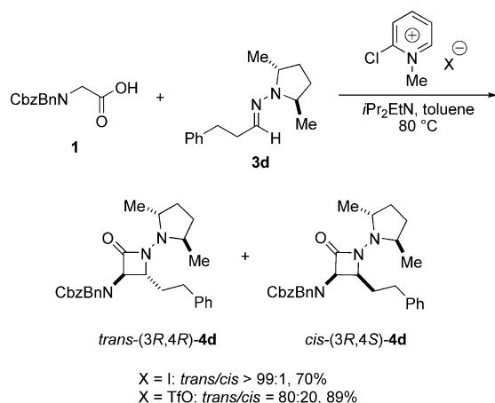
Scheme 4. Effect of nucleophiles on the trans/cis ratio of the cycloaddition.
