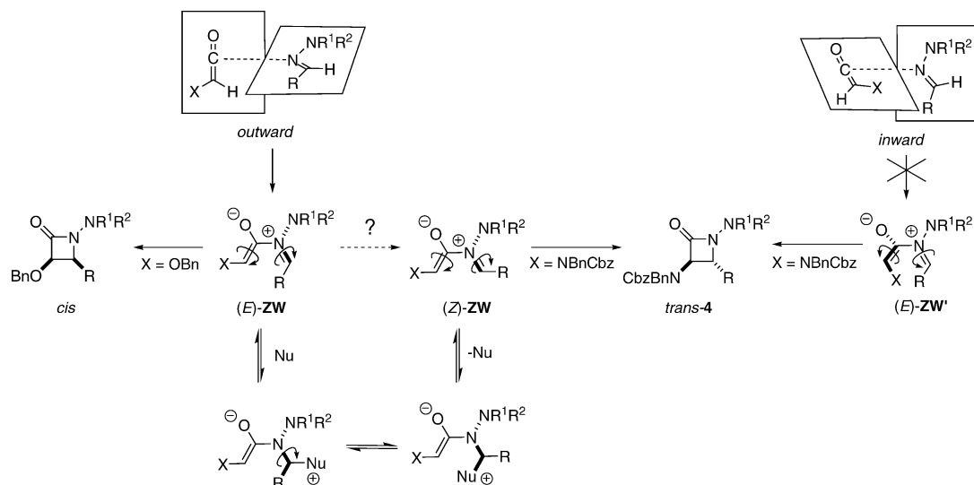
Scheme 3. Suggested model for the relative stereochemistry of the cycloaddition.
