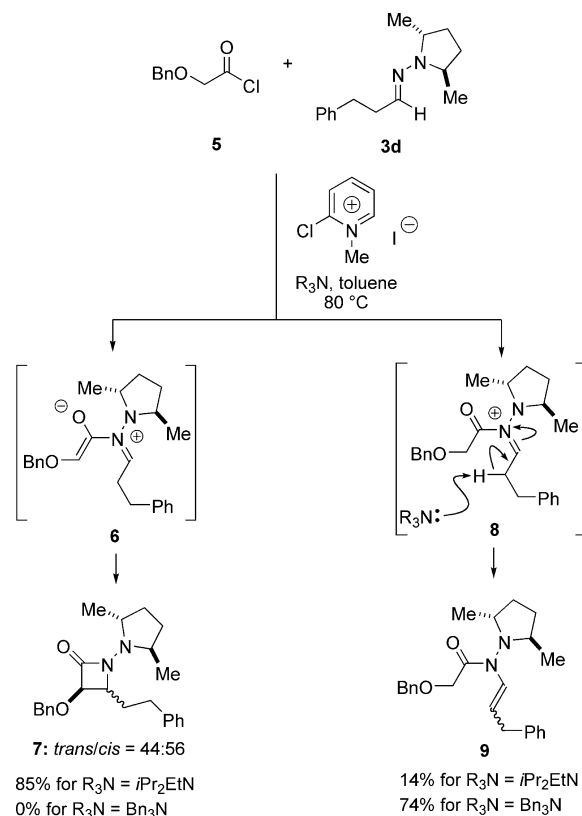
Scheme 5. Reaction of hydrazone 3d with benzyloxyacetyl chloride 5 .
