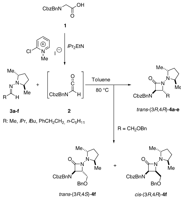
Scheme 2. Synthesis of 3-amino-4-alkylazetidin-2-ones 4 .
