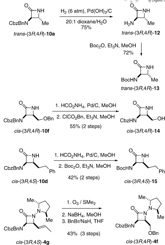
Scheme 8. Chemical correlations used for the determination of the absolute configurations.
