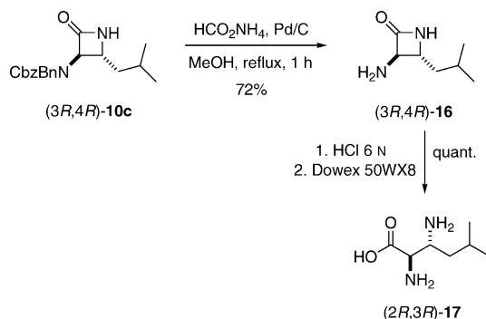
Scheme 9. Synthesis of \alpha,\beta -diamino acid (2 R ,3 R )- 17 .
