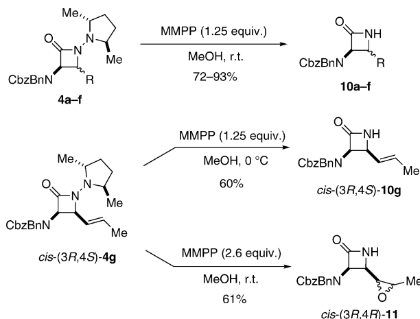
Scheme 7. Release of the chiral auxiliary: oxidative cleavage of the \text{N–N} bond.
