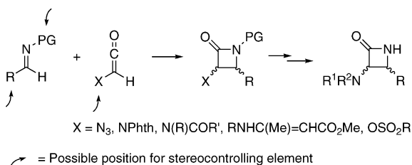
Scheme 1. The ketene-imine [2+2] cycloaddition approach to 3-amino-β-lactams.
