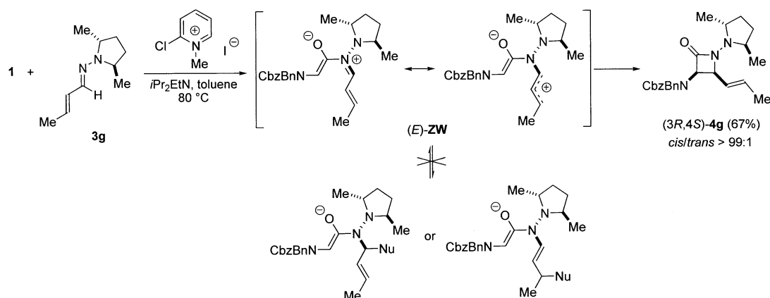
Scheme 6. Reaction of crotonaldehyde derivative 3g with N -benzyl- N -(benzyloxycarbonyl)glycine ( 1 ).
